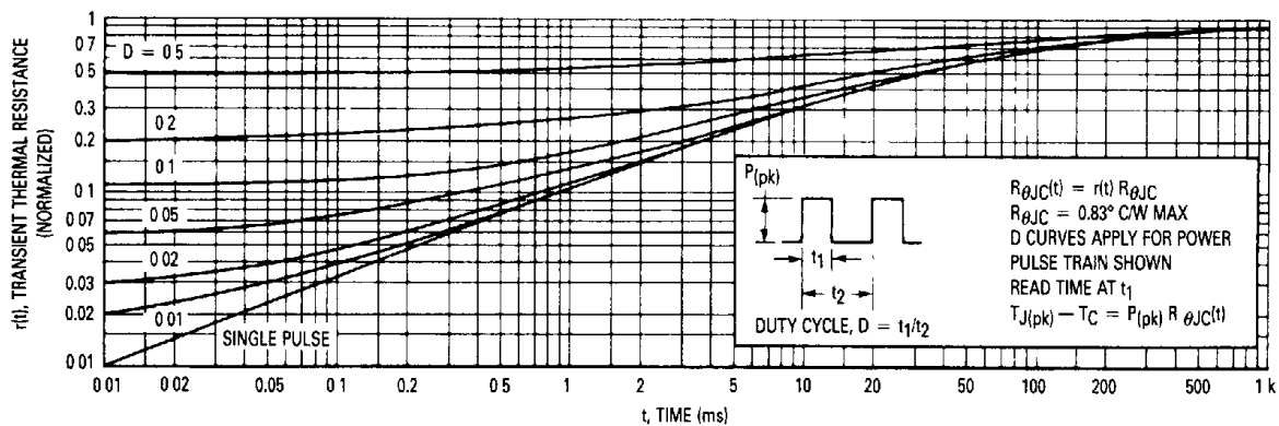
Figure 10. Thermal Response
